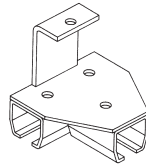
Track Bracket 3 Way Threaded Rod Part 10291
